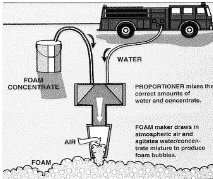
After the foam concentrate has been mixed with water to form a foam solution, it must be aerated to form (finished) foam.
